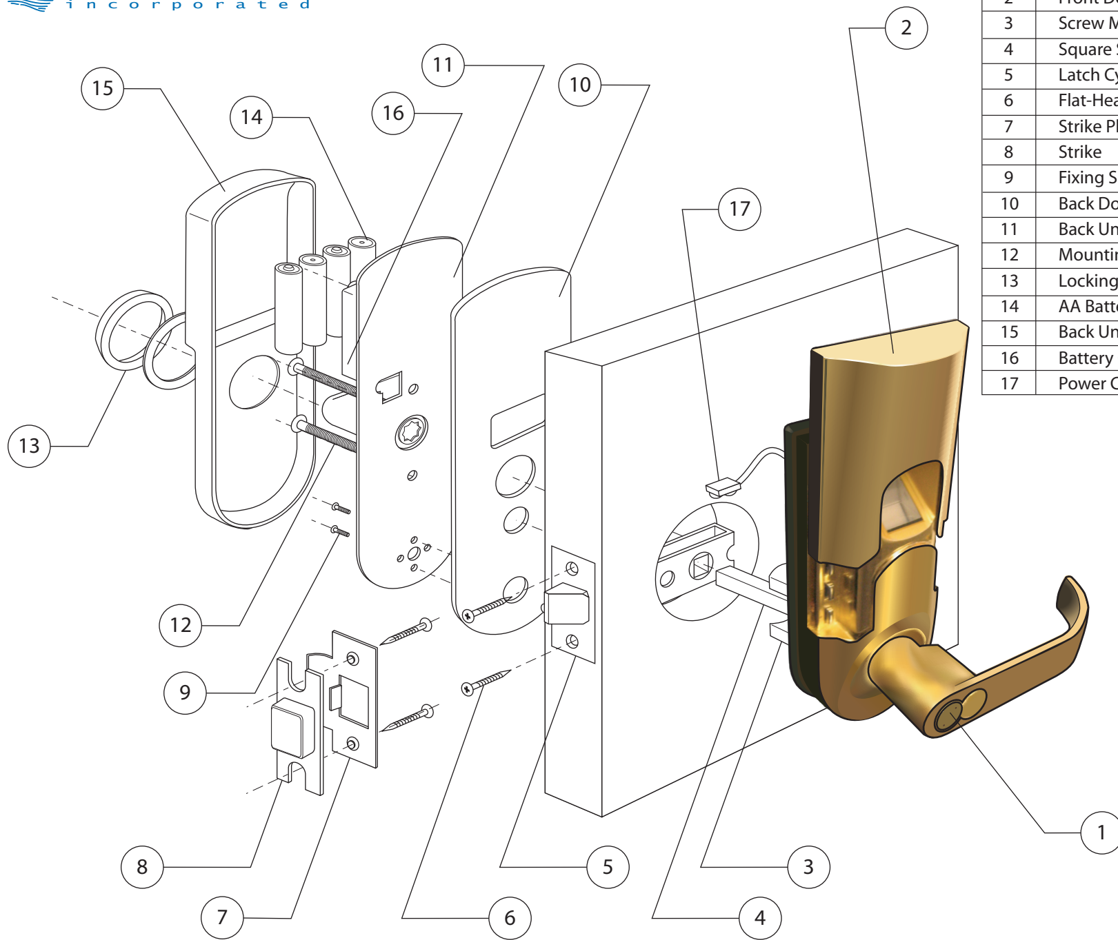
DIGI 86 Door Lock Series Assembly Drawing
